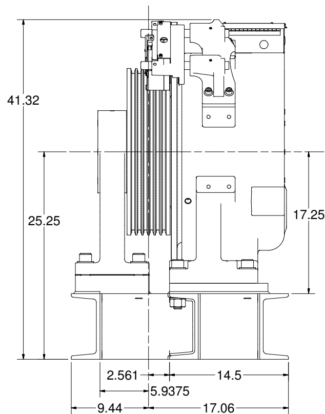
20" TRACTION WHEEL
