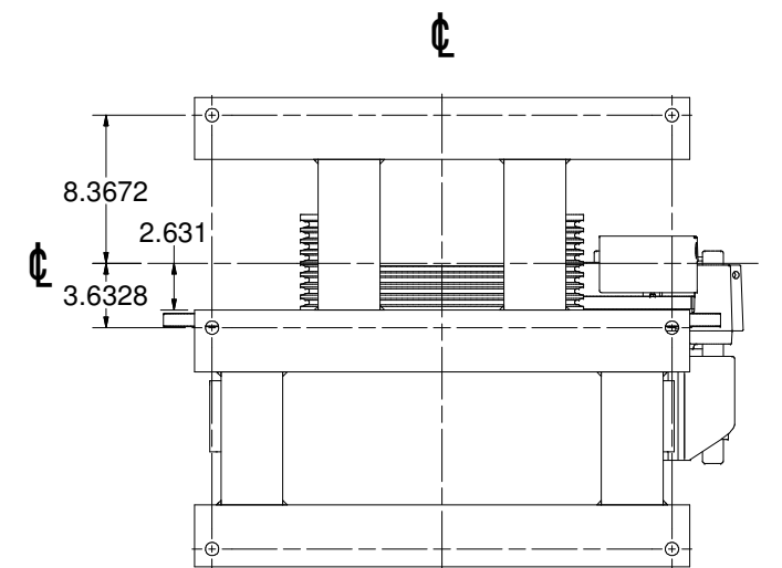
VIEW C-C SCALE 1 / 6 15.75" TW
