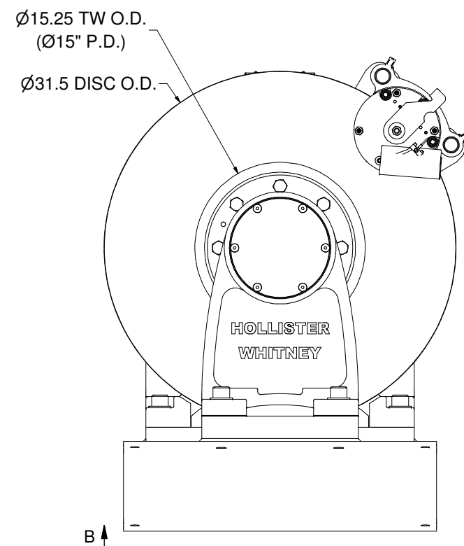
15" TRACTION WHEEL
