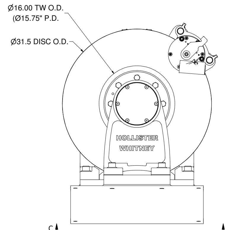
15.75" TRACTION WHEEL
