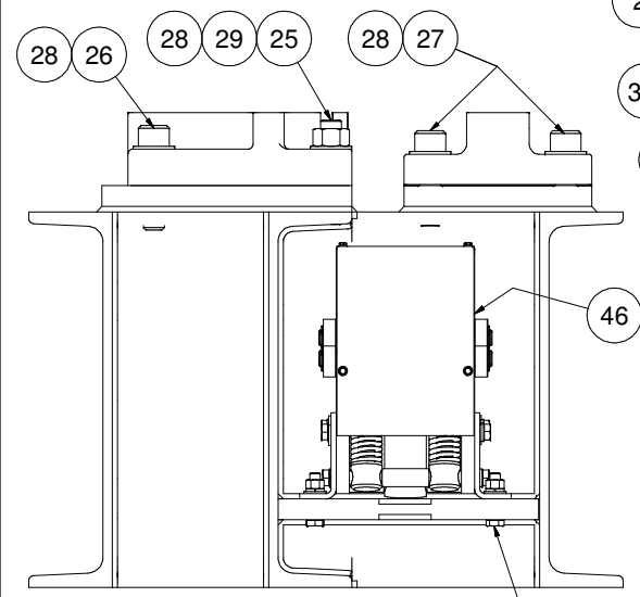
VIEW B-B
