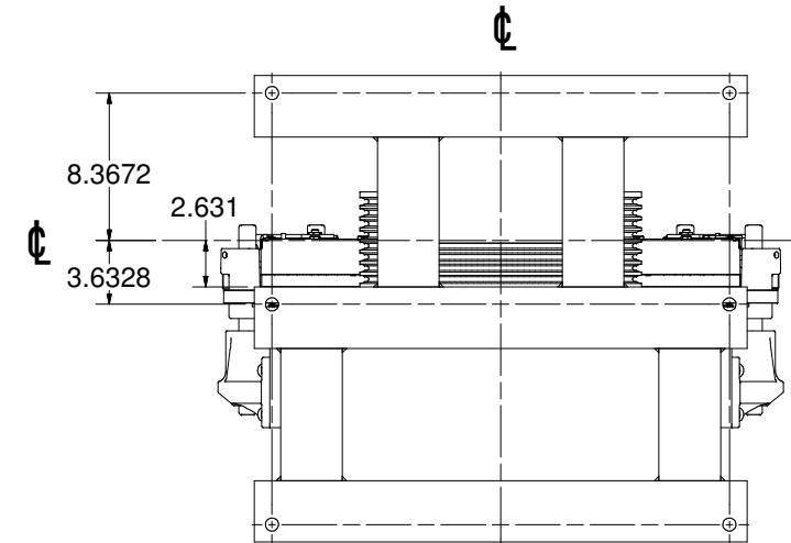
VIEW C-C SCALE 1 / 6 15.75" TW
