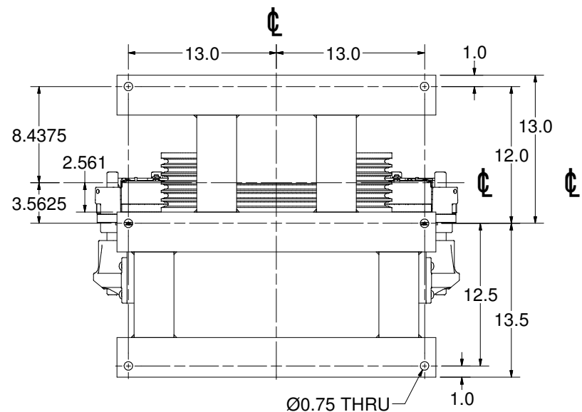
VIEW A-A SCALE 1 / 6 20" TW
