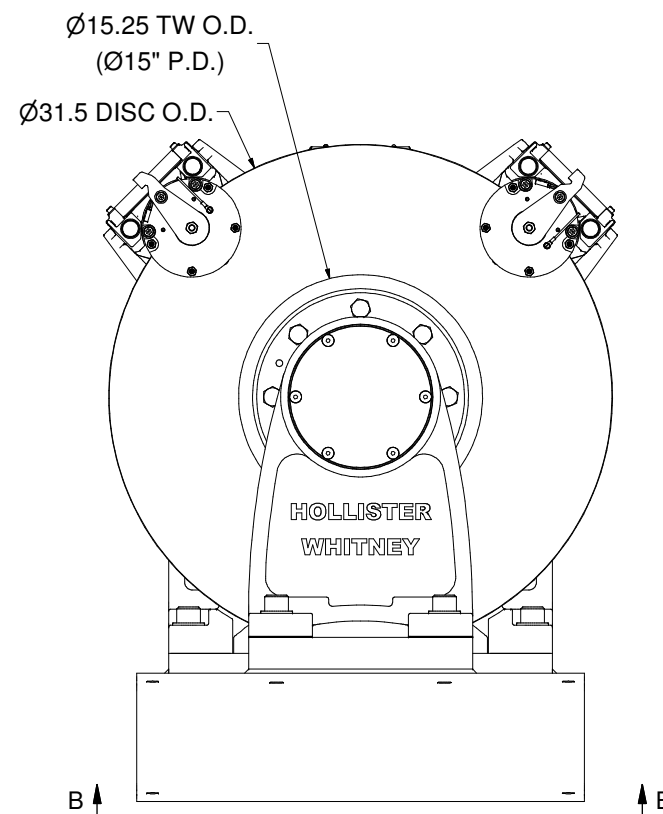
15" TRACTION WHEEL
