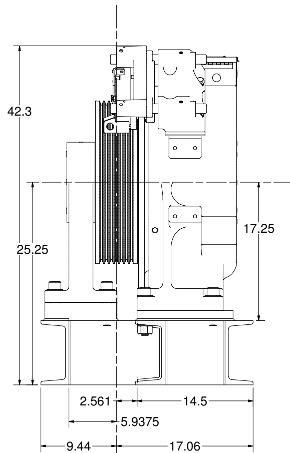
VIEW A-A SCALE 1 / 6 20" TW
