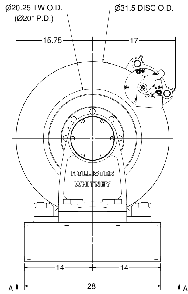
20" TRACTION WHEEL
