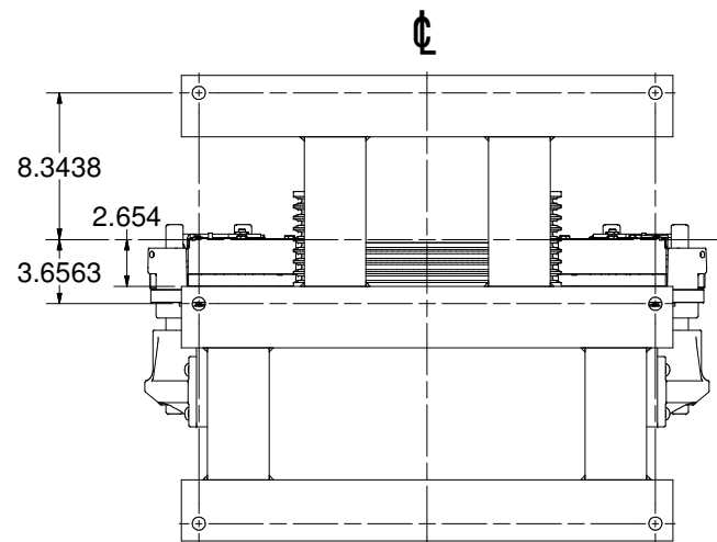
VIEW B-B SCALE 1 / 6 15" TW
