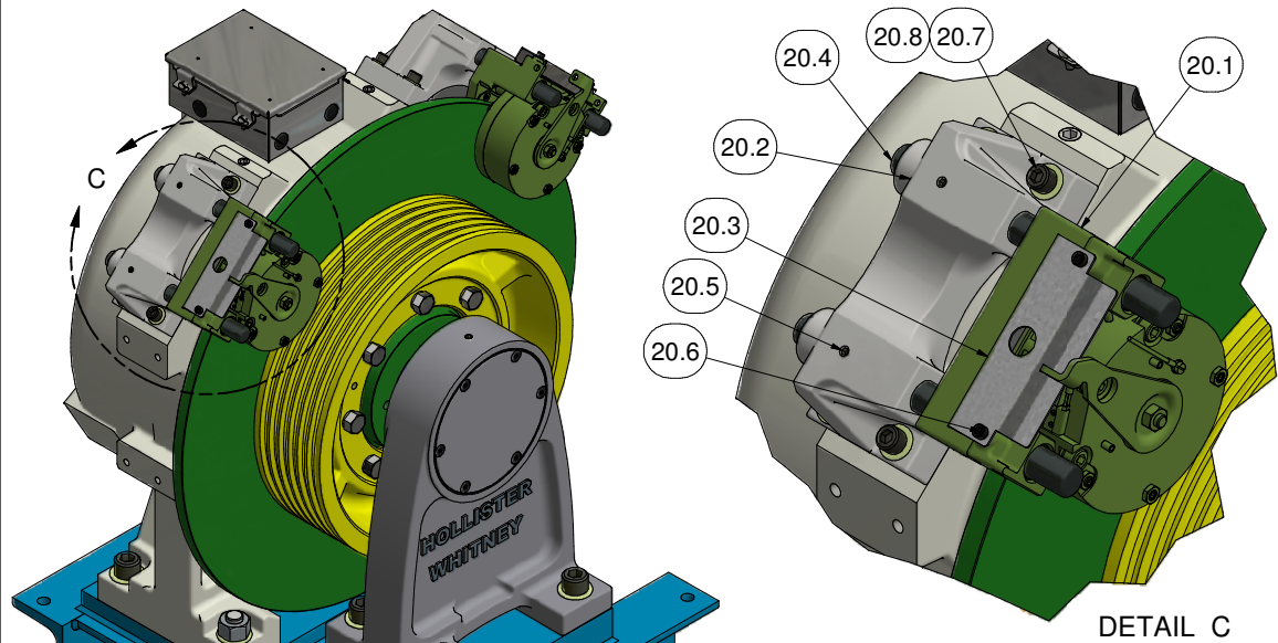
DETAIL C
