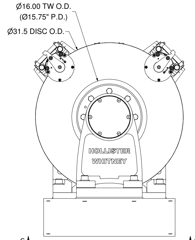
15.75" TRACTION WHEEL
