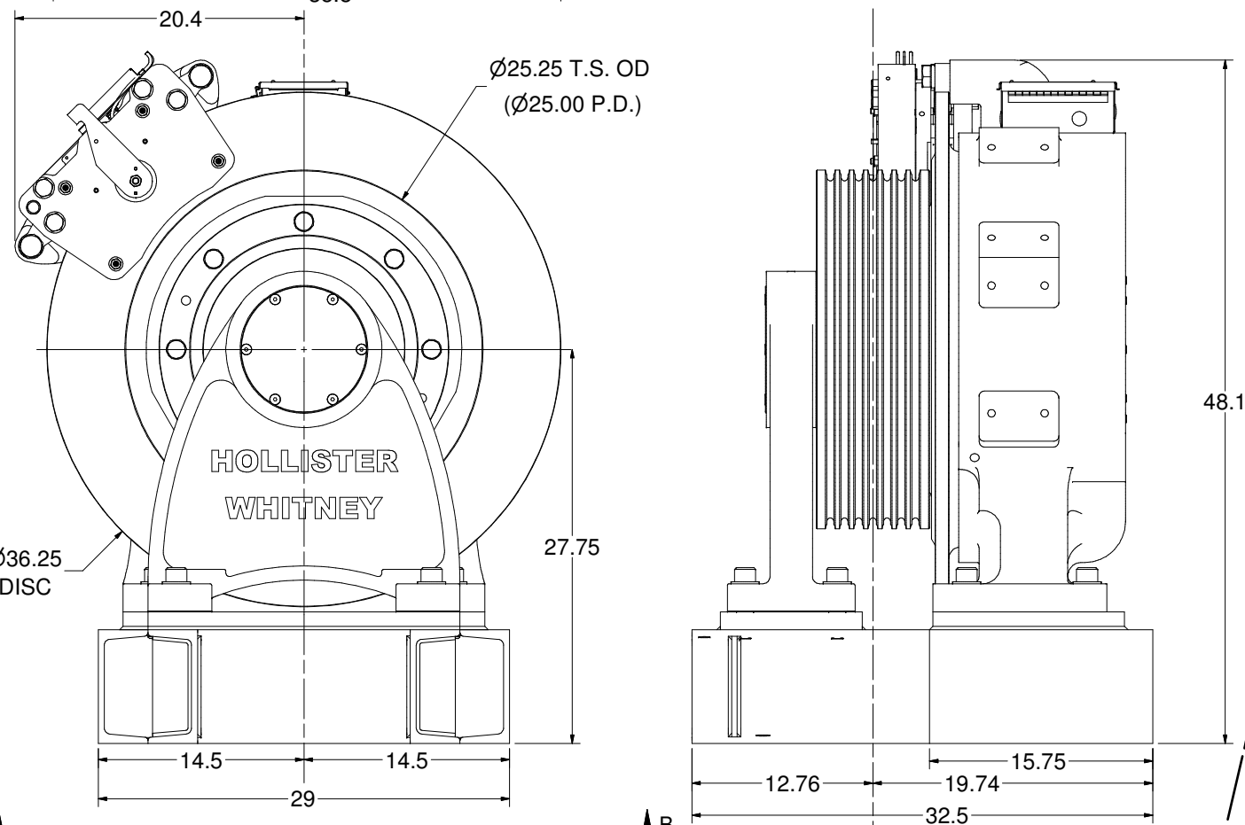
25" SHEAVE 2000# CAP. MAX GL130A Mass: 3828 lbmass
