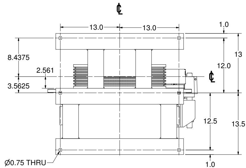
VIEW A-A SCALE 1 / 6 20" TW
