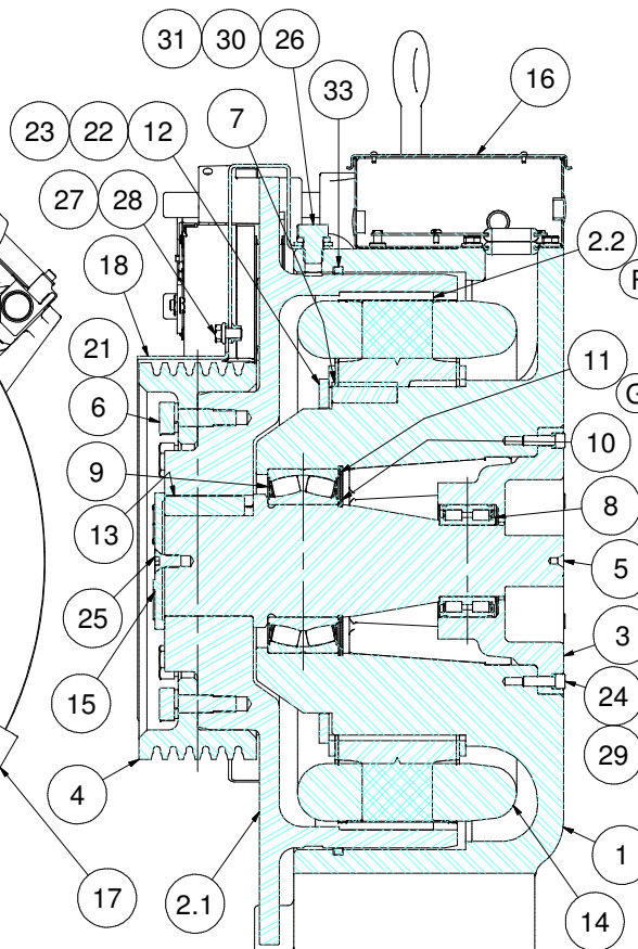
SECTION A-A SCALE 1 / 4
